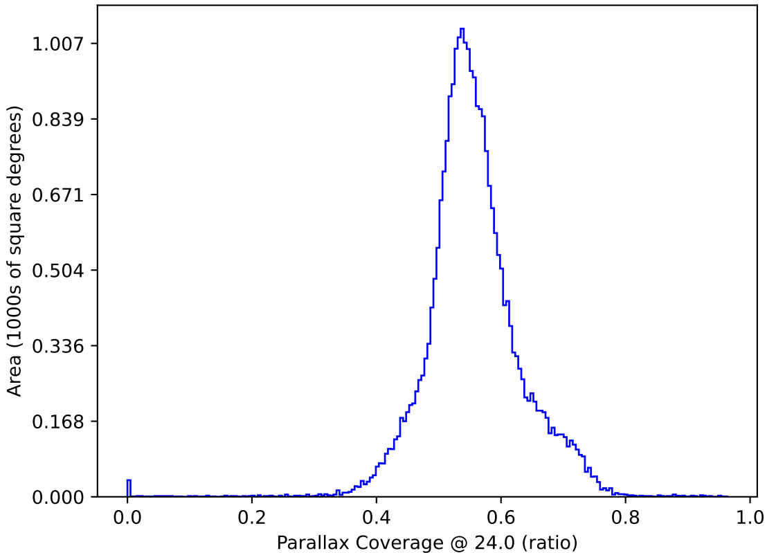
ddf_loaded_fl1_v3.3_10yrs : Parallax Coverage @ 24.0
