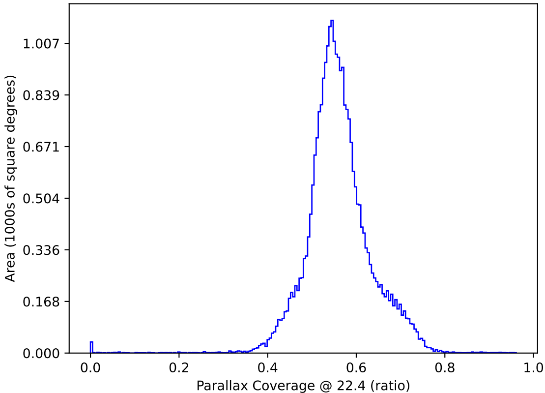
ddf_loaded_fl1_v3.3_10yrs : Parallax Coverage @ 22.4
