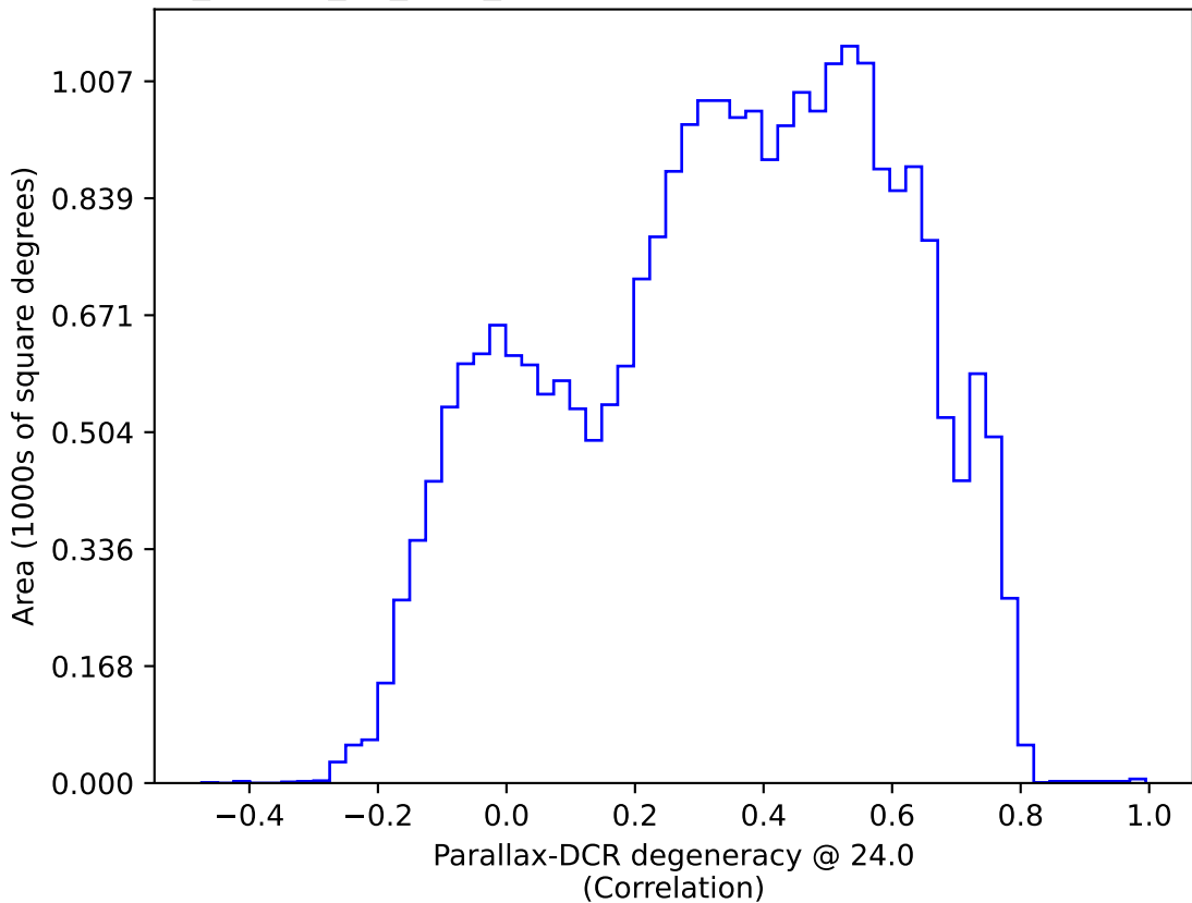
ddf_loaded_fl1_v3.3_10yrs : Parallax-DCR degeneracy @ 24.0
