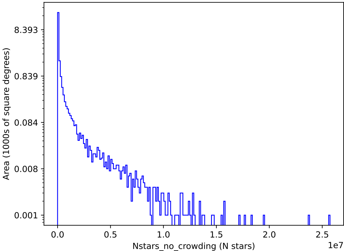
ddf_loaded_fl1_v3.3_10yrs y: Nstars_no_crowding
