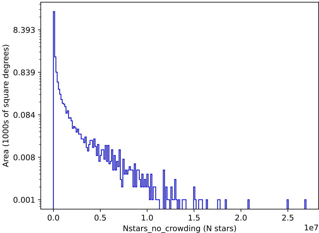
ddf_loaded_fl1_v3.3_10yrs i: Nstars_no_crowding
