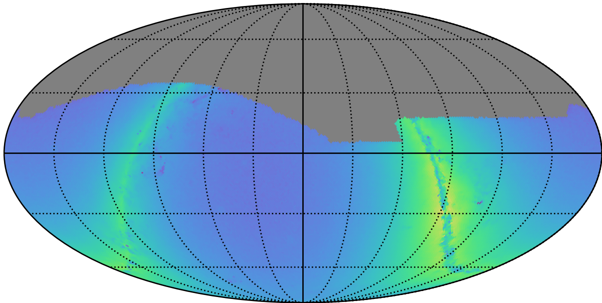
ddf_loaded_fl1_v3.3_10yrs g: Nstars_no_crowding
