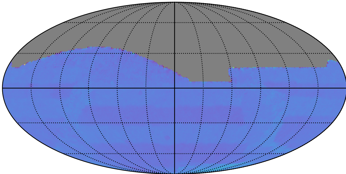
ddf_loaded_fl1_v3.3_10yrs : Normalized Proper Motion Uncert @ 20.5
