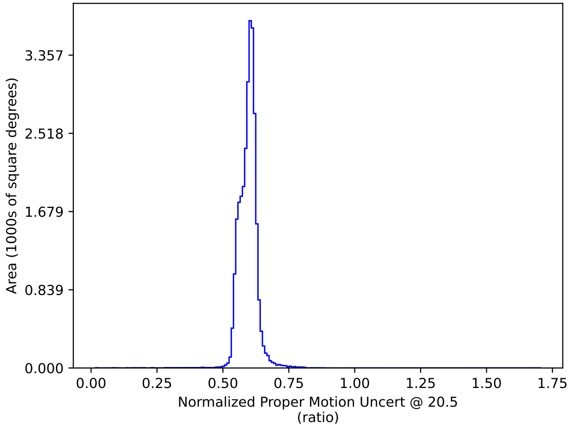
ddf_loaded_fl1_v3.3_10yrs : Normalized Proper Motion Uncert @ 20.5
