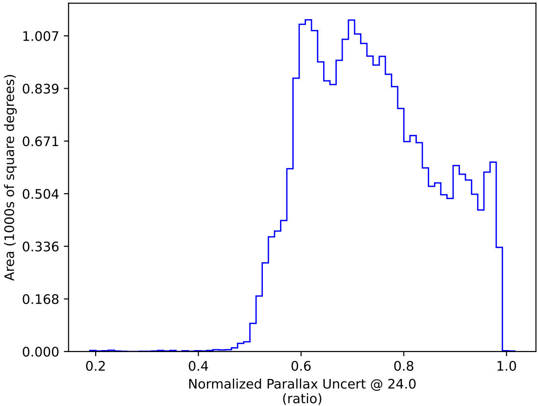
ddf_loaded_fl1_v3.3_10yrs : Normalized Parallax Uncert @ 24.0
