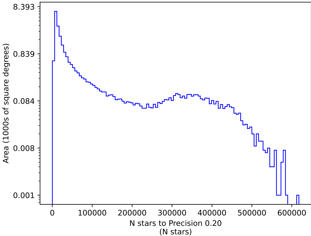
ddf_loaded_fl1_v3.3_10yrs y: N stars to Precision 0.20
