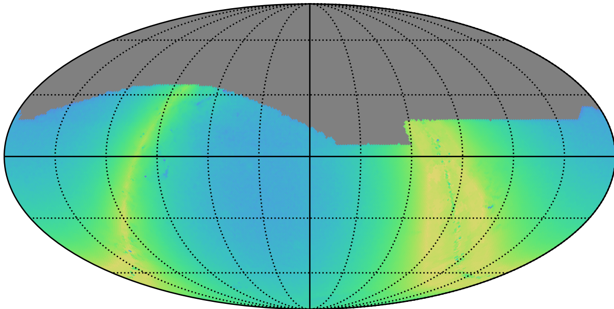
ddf_loaded_fl1_v3.3_10yrs r: N stars to Precision 0.20
