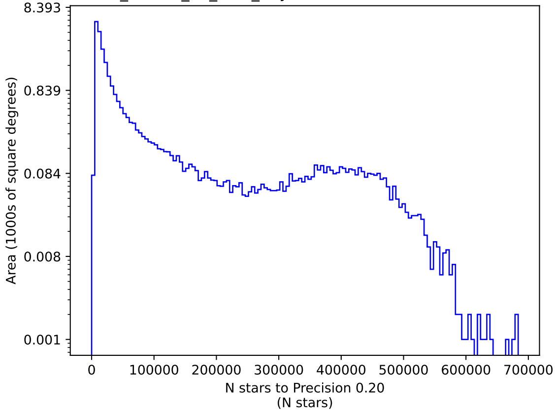
ddf_loaded_fl1_v3.3_10yrs i: N stars to Precision 0.20
