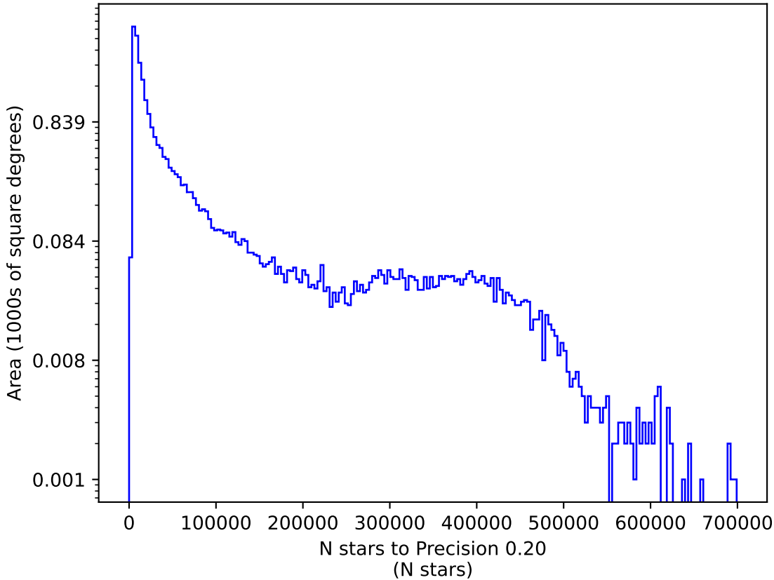
ddf_loaded_fl1_v3.3_10yrs g: N stars to Precision 0.20
