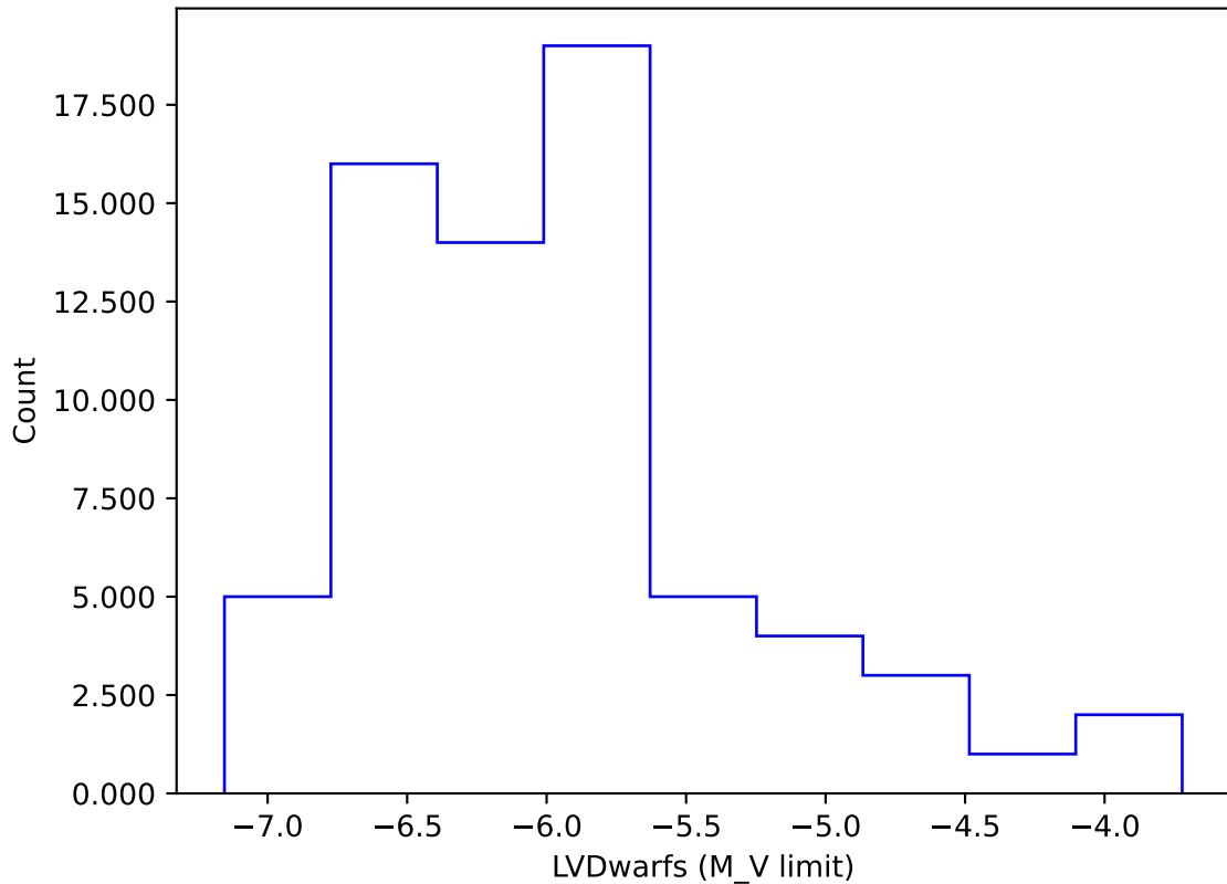
ddf_loaded_fl1_v3.3_10yrs gi: LVDwarfs
