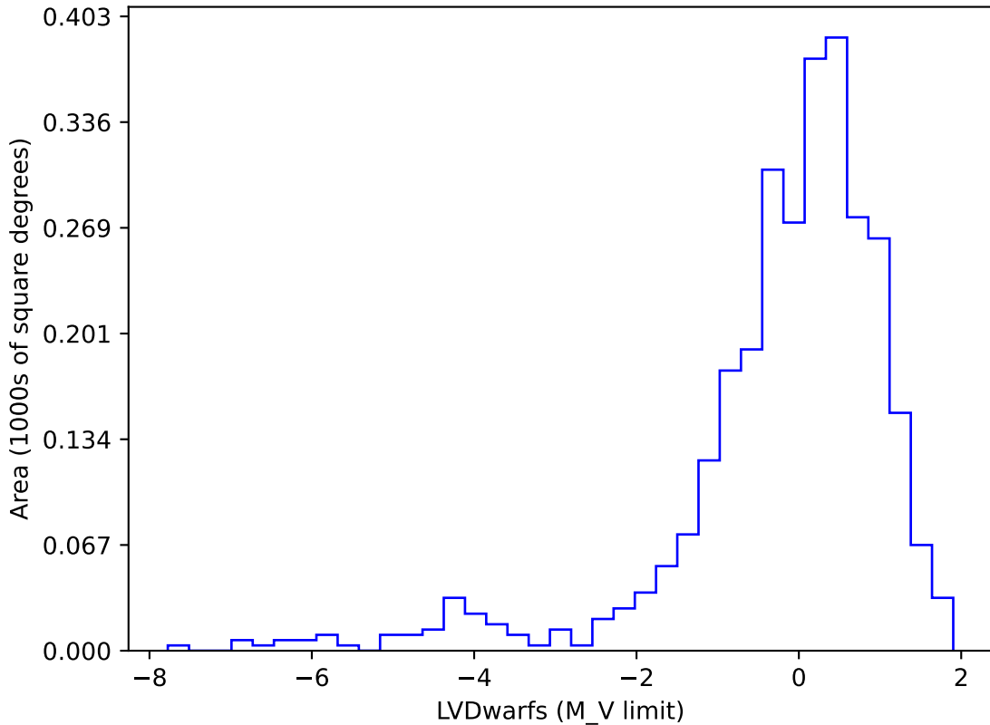
ddf_loaded_fl1_v3.3_10yrs gi SCP: LVDwarfs
