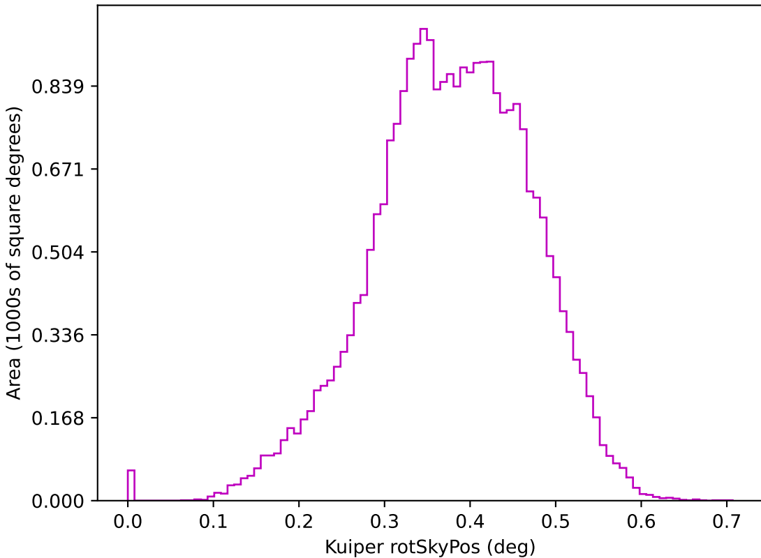
ddf_loaded_fl1_v3.3_10yrs z: Kuiper rotSkyPos
