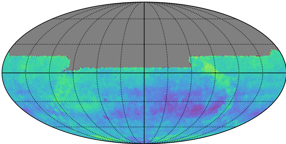
ddf_loaded_fl1_v3.3_10yrs y: Kuiper rotSkyPos
