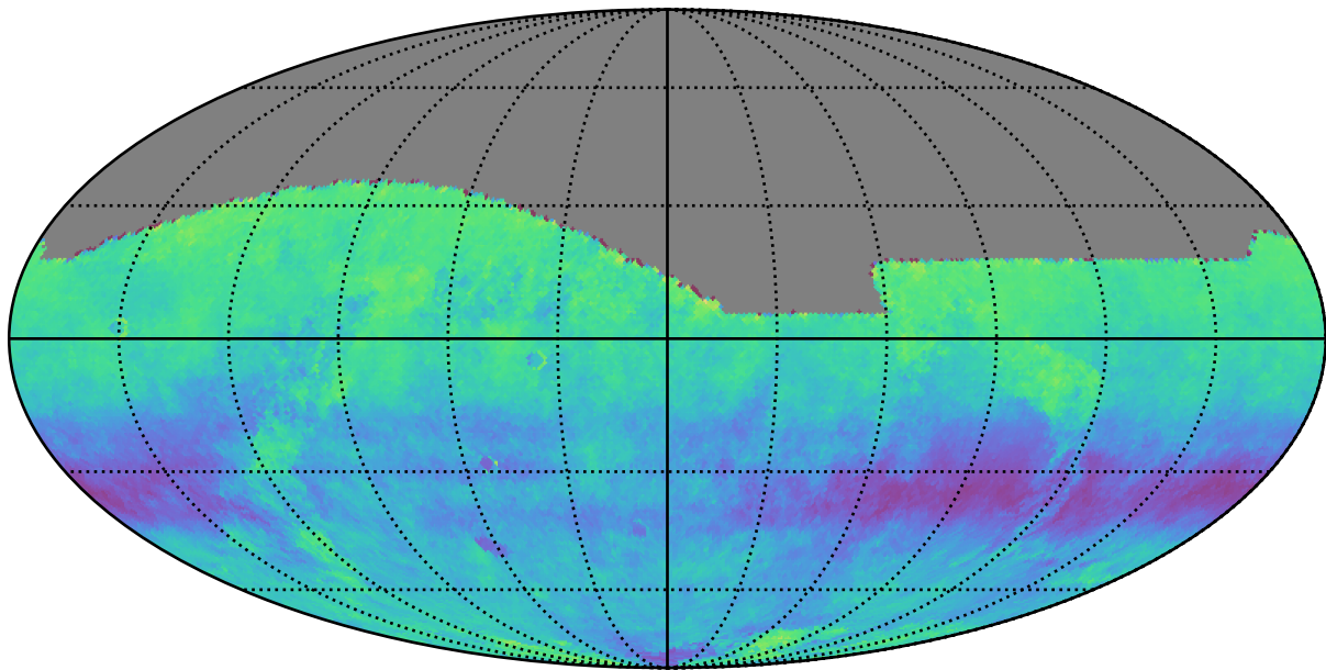
ddf_loaded_fl1_v3.3_10yrs r: Kuiper rotSkyPos
