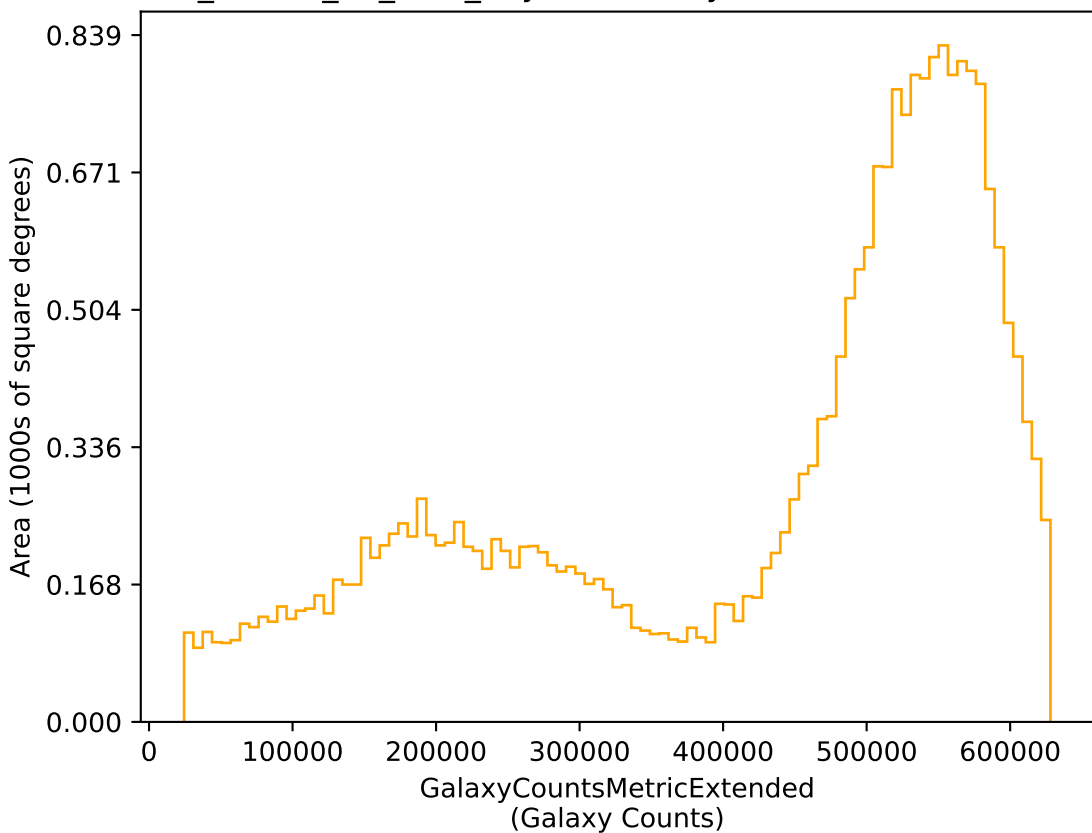
ddf_loaded_fl1_v3.3_10yrs r: GalaxyCountsMetricExtended
