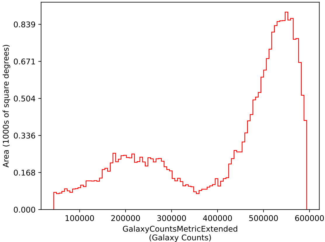
ddf_loaded_fl1_v3.3_10yrs i: GalaxyCountsMetricExtended
