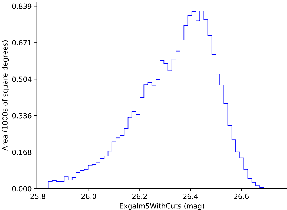
ddf_loaded_fl1_v3.3_10yrs i band non-DD year 9: ExgalM5WithCuts
