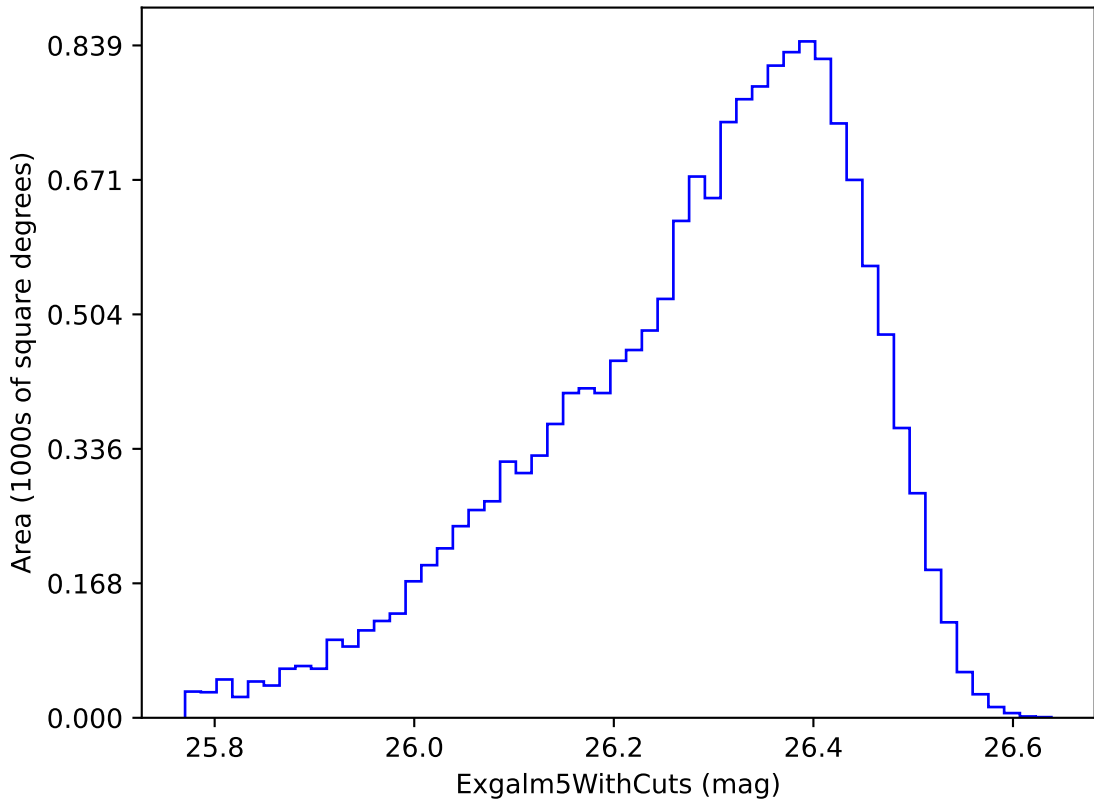
ddf_loaded_fl1_v3.3_10yrs i band non-DD year 8: ExgalM5WithCuts
