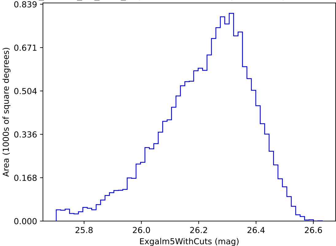
ddf_loaded_fl1_v3.3_10yrs i band non-DD year 7: Exgal5WithCuts
