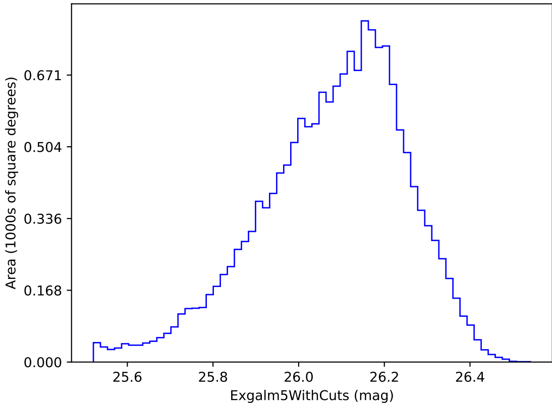
ddf_loaded_fl1_v3.3_10yrs i band non-DD year 5: ExgalM5WithCuts
