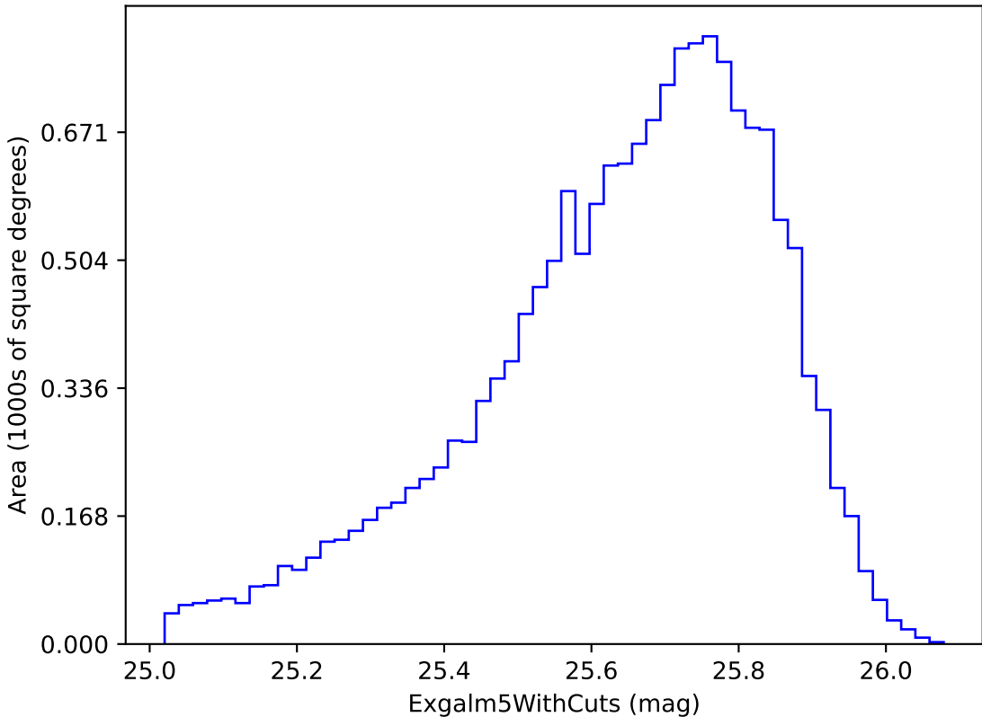
ddf_loaded_fl1_v3.3_10yrs i band non-DD year 2: ExgalM5WithCuts
