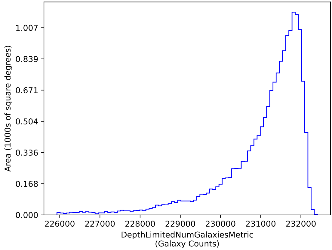
ddf_loaded_fl1_v3.3_10yrs i band galaxies non-DD: DepthLimitedNumGalaxiesMetric
