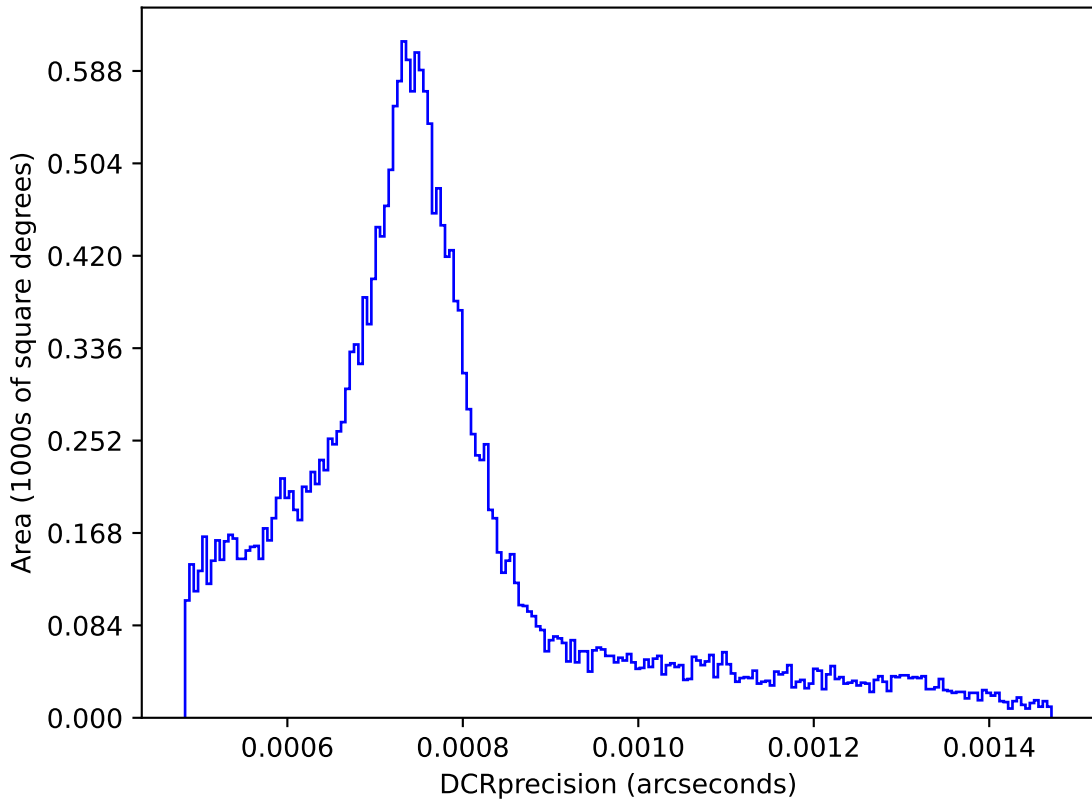
ddf_loaded_fl1_v3.3_10yrs : DCRprecision
