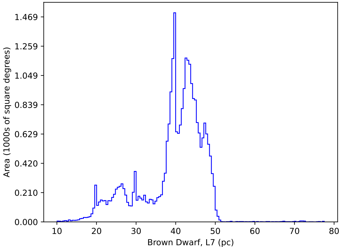
ddf_loaded_fl1_v3.3_10yrs : Brown Dwarf, L7
