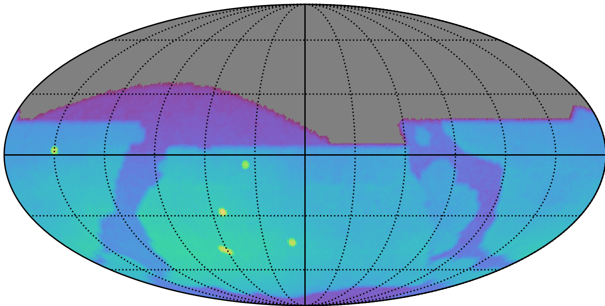
ddf_loaded_fl1_v3.3_10yrs : Brown Dwarf, L4
