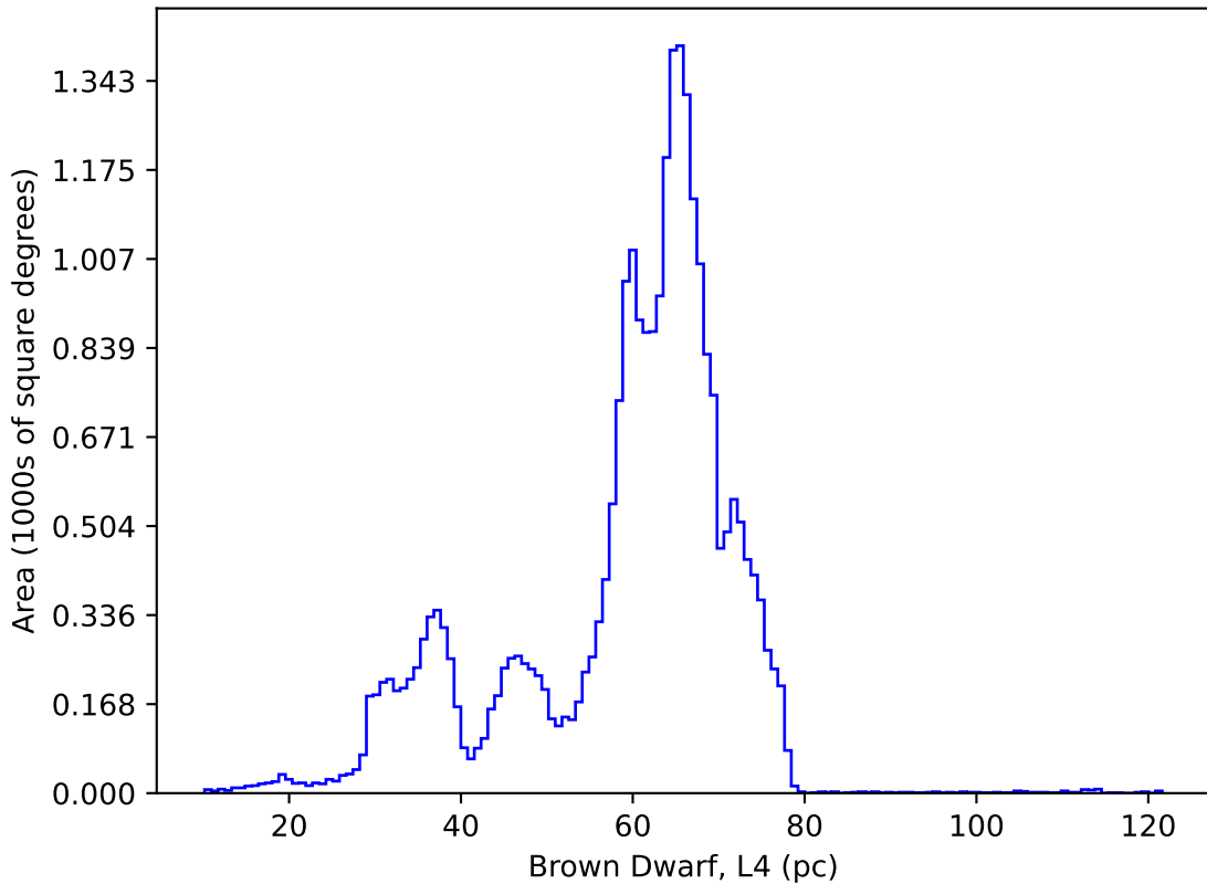
ddf_loaded_fl1_v3.3_10yrs : Brown Dwarf, L4
