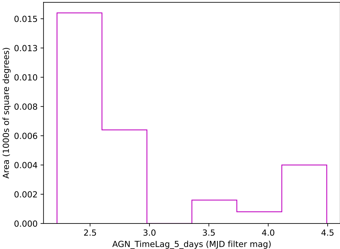
ddf_loaded_fl1_v3.3_10yrs z band: AGN_TimeLag_5_days
