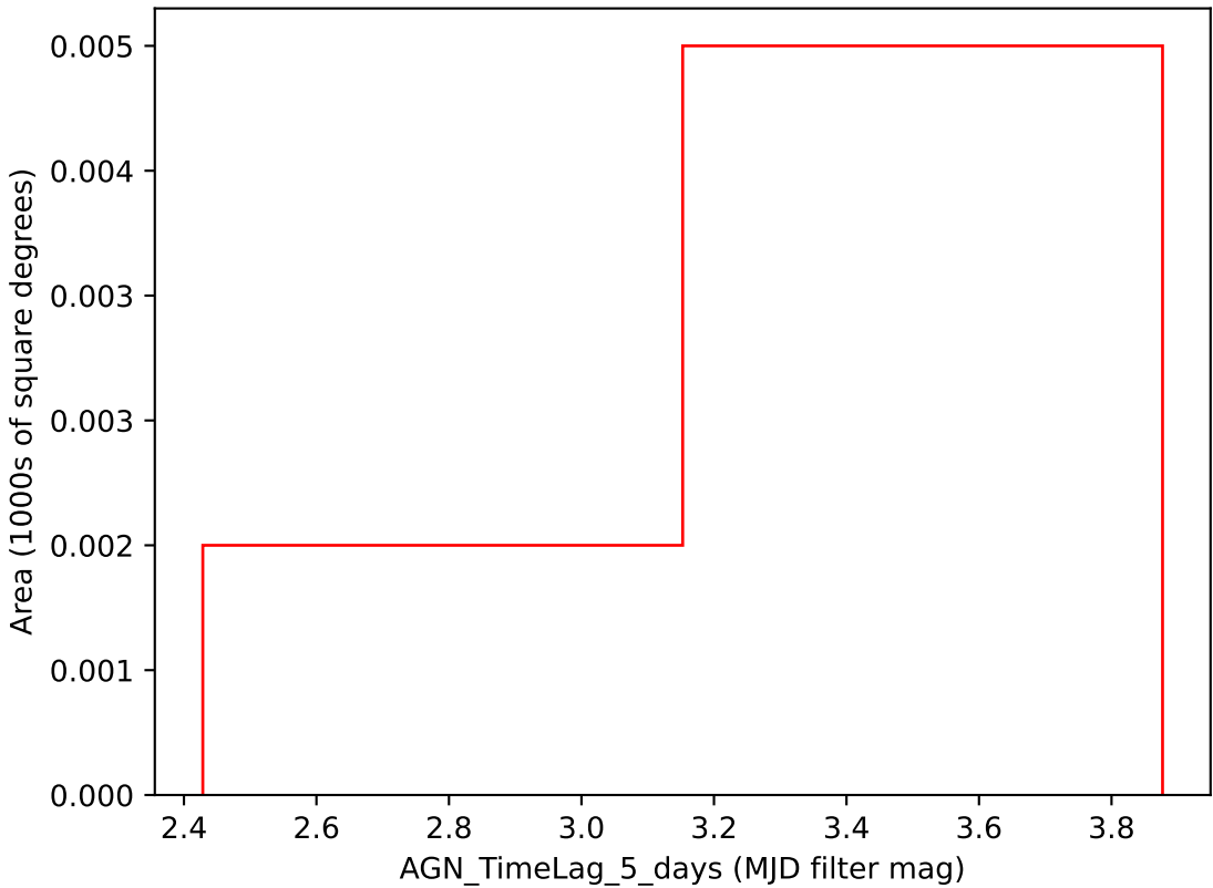
ddf_loaded_fl1_v3.3_10yrs i band: AGN_TimeLag_5_days
