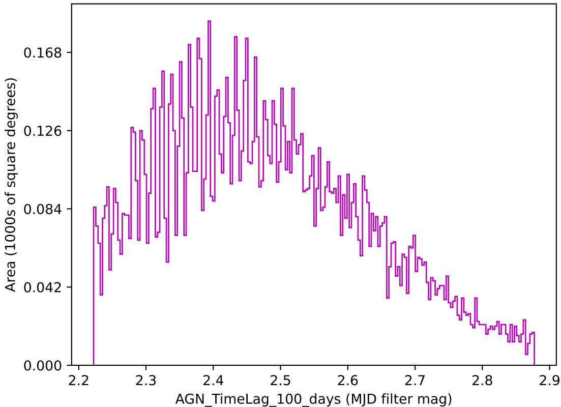
ddf_loaded_fl1_v3.3_10yrs z band: AGN_TimeLag_100_days
