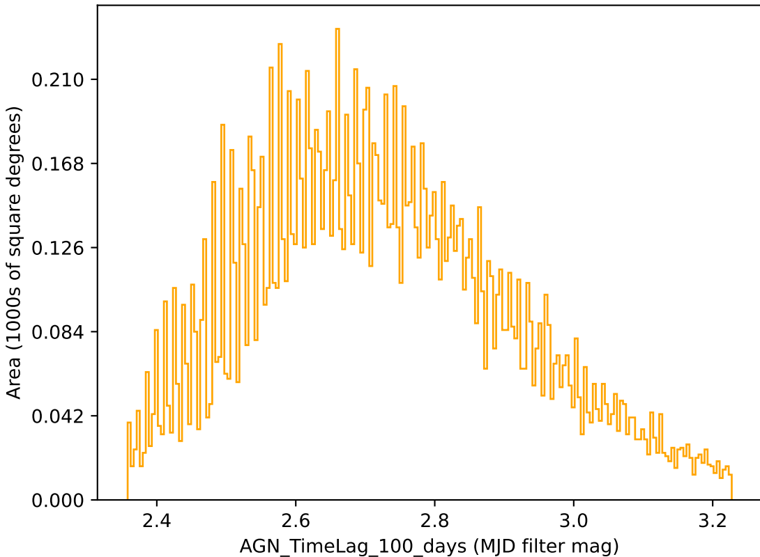
ddf_loaded_fl1_v3.3_10yrs r band: AGN_TimeLag_100_days
