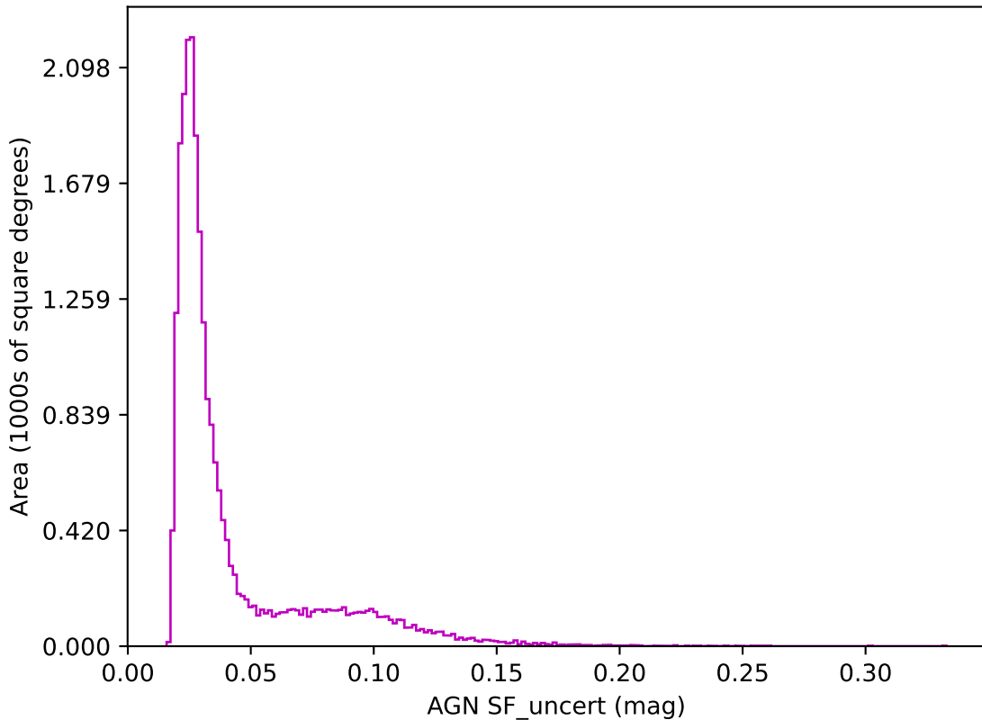
ddf_loaded_fl1_v3.3_10yrs z band: AGN SF_uncert
