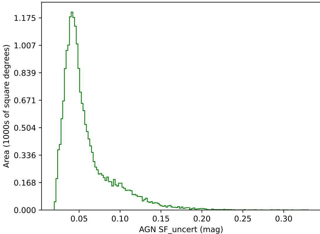
ddf_loaded_fl1_v3.3_10yrs g band: AGN SF_uncert
