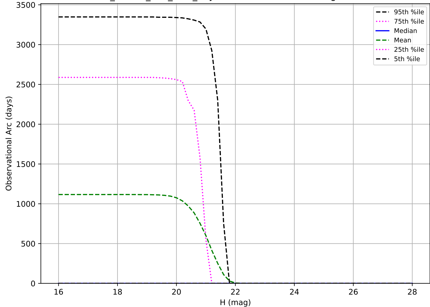
ddf_loaded_fl15_v3.4_10yrs: Observational Arc Length Vatira
