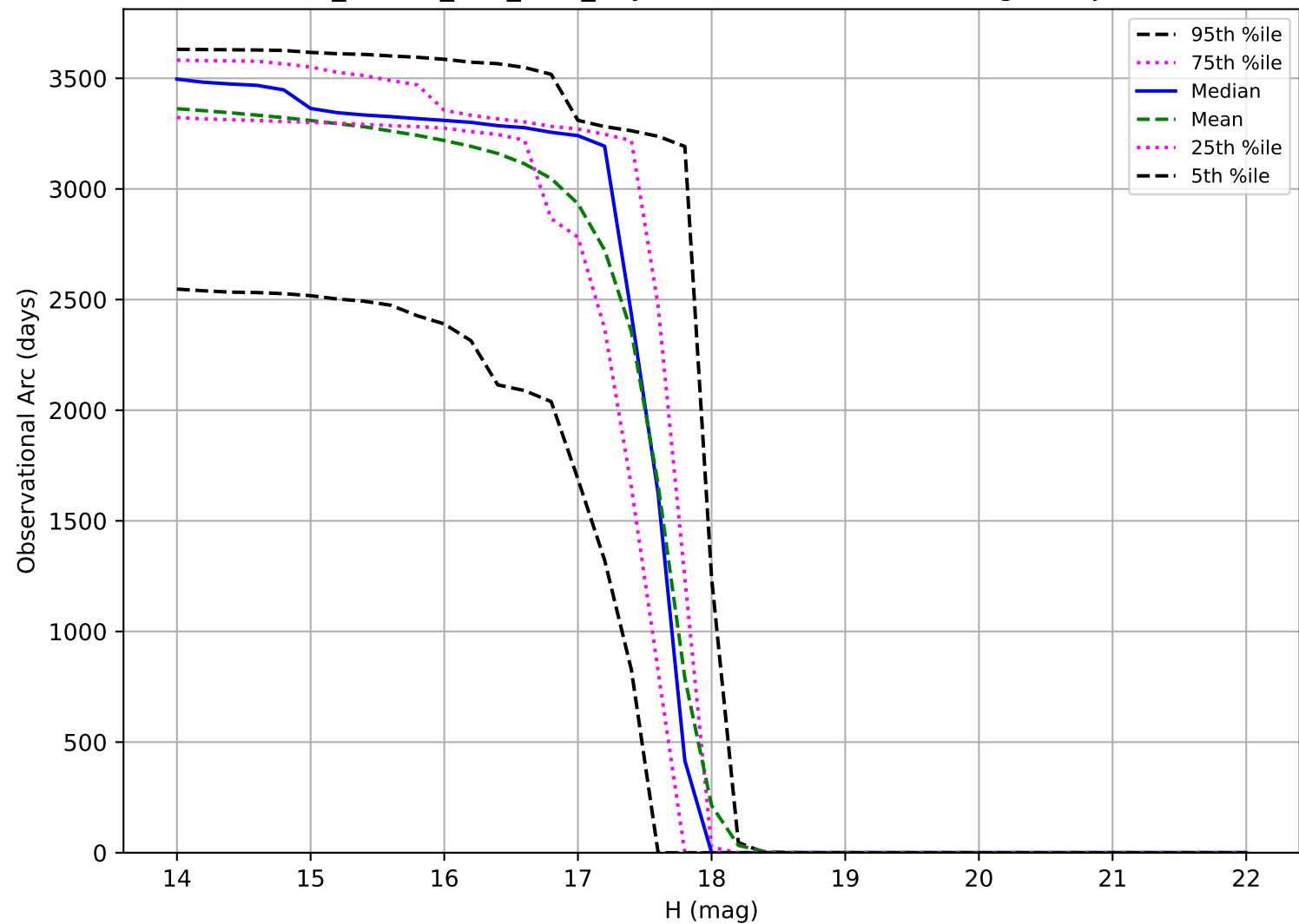
ddf_loaded_fl15_v3.4_10yrs: Observational Arc Length Trojan
