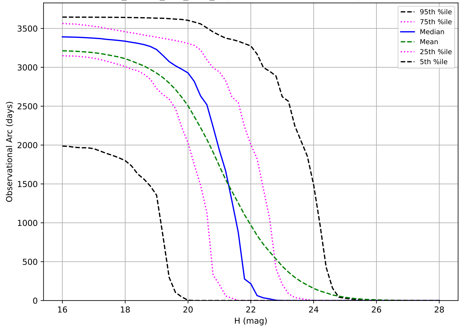
ddf_loaded_fl15_v3.4_10yrs: Observational Arc Length PHA
