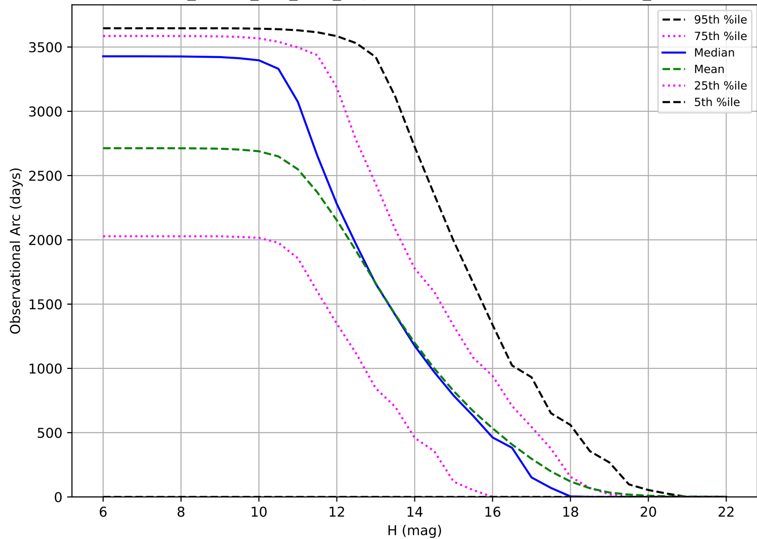
ddf_loaded_fl15_v3.4_10yrs: Observational Arc Length OCC_r5
