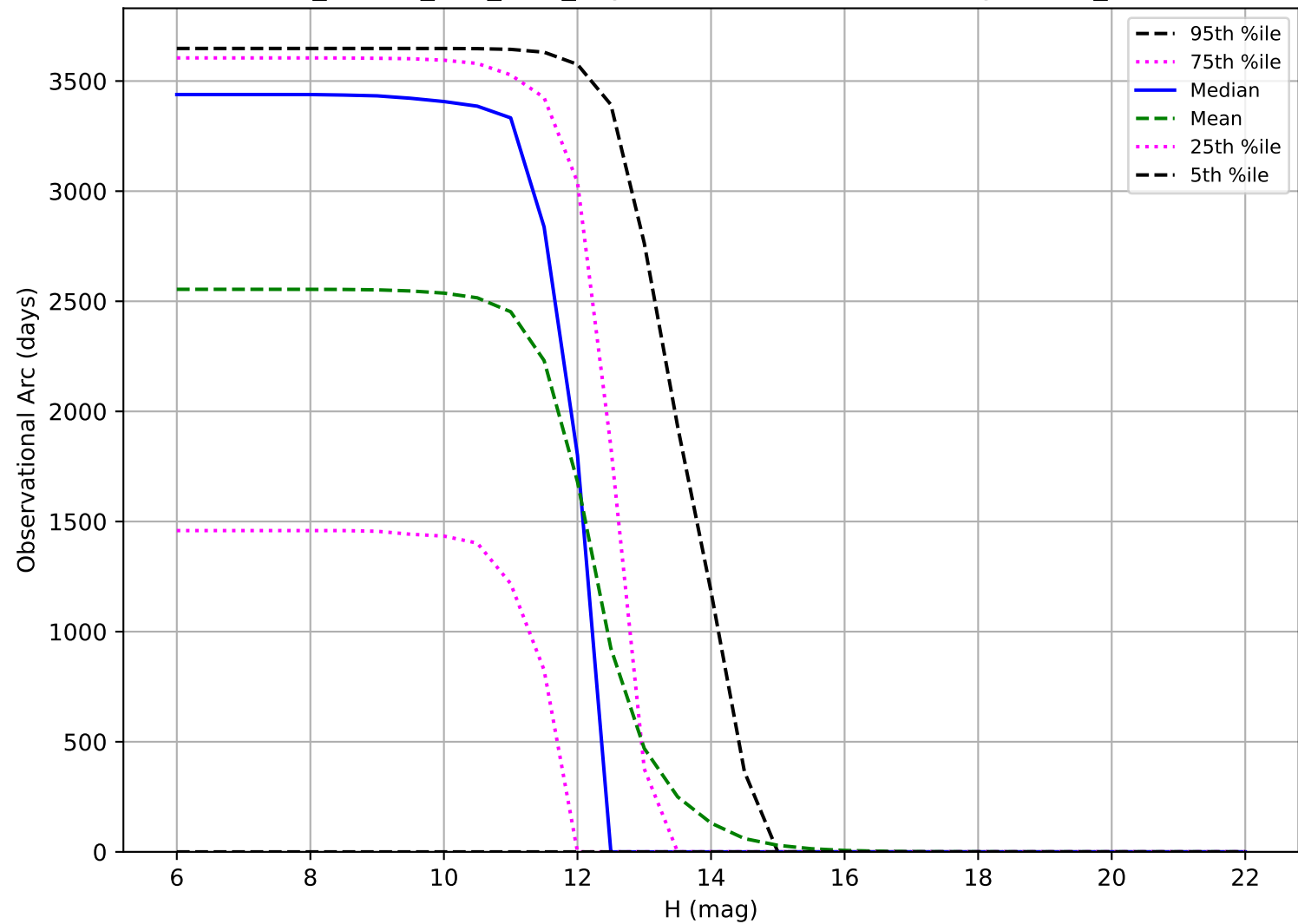
ddf_loaded_fl15_v3.4_10yrs: Observational Arc Length OCC_r20
