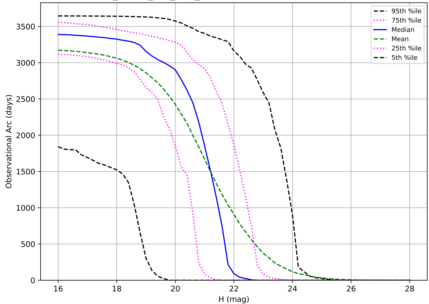
ddf_loaded_fl15_v3.4_10yrs: Observational Arc Length NEO
