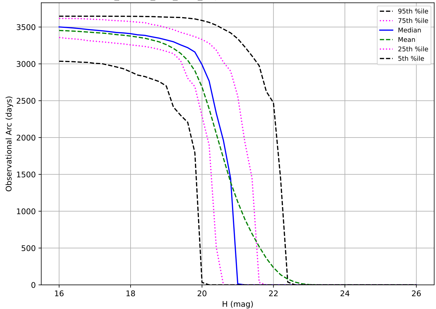
ddf_loaded_fl15_v3.4_10yrs: Observational Arc Length MBA
