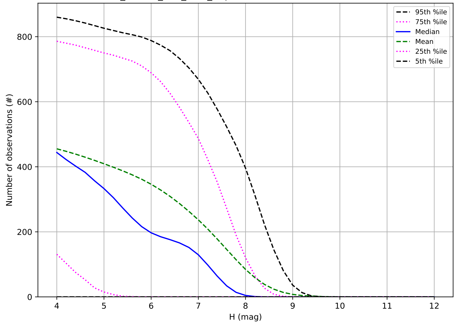
ddf_loaded_fl15_v3.4_10yrs: Number of observations TNO
