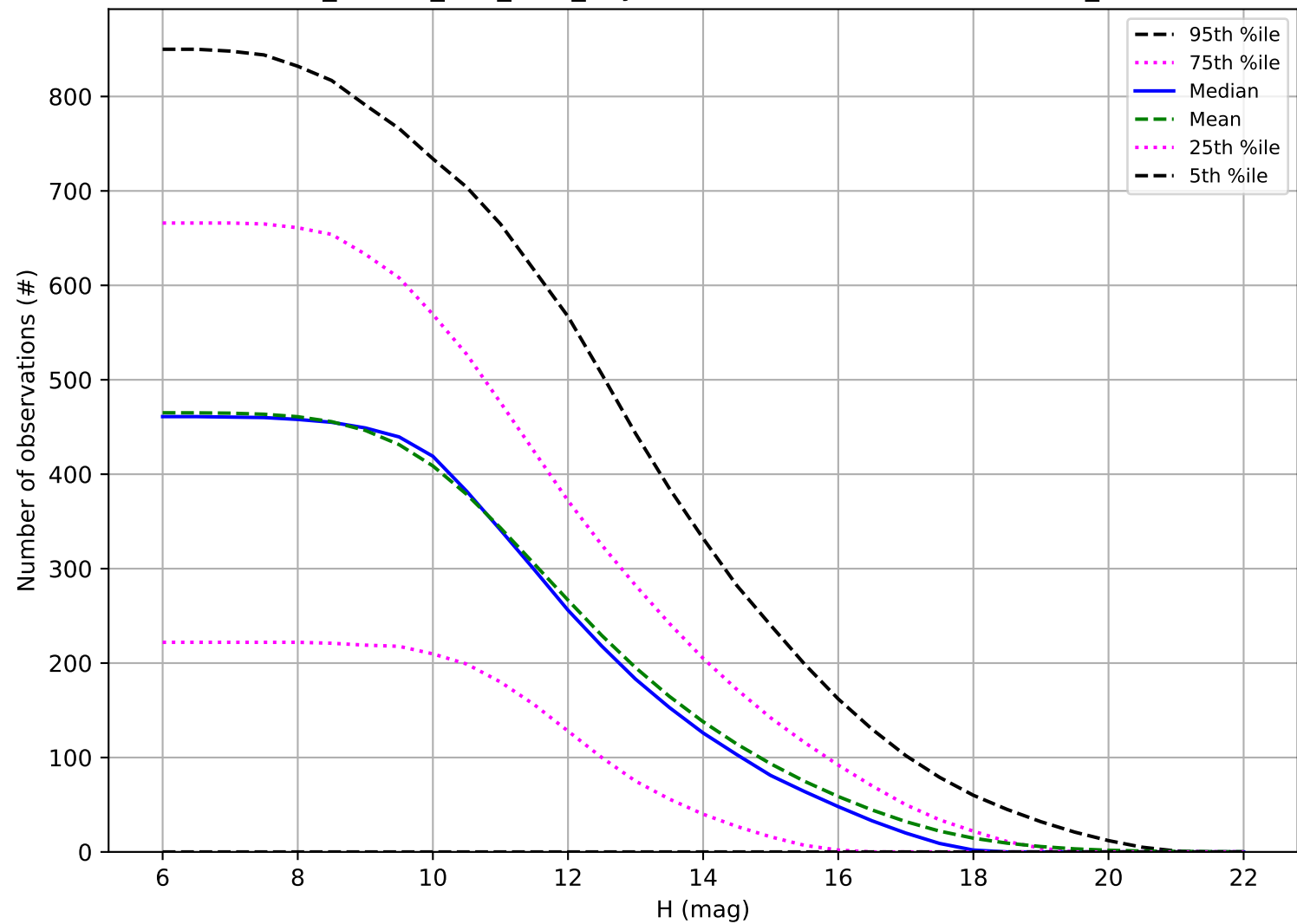
ddf_loaded_fl15_v3.4_10yrs: Number of observations OCC_r5
