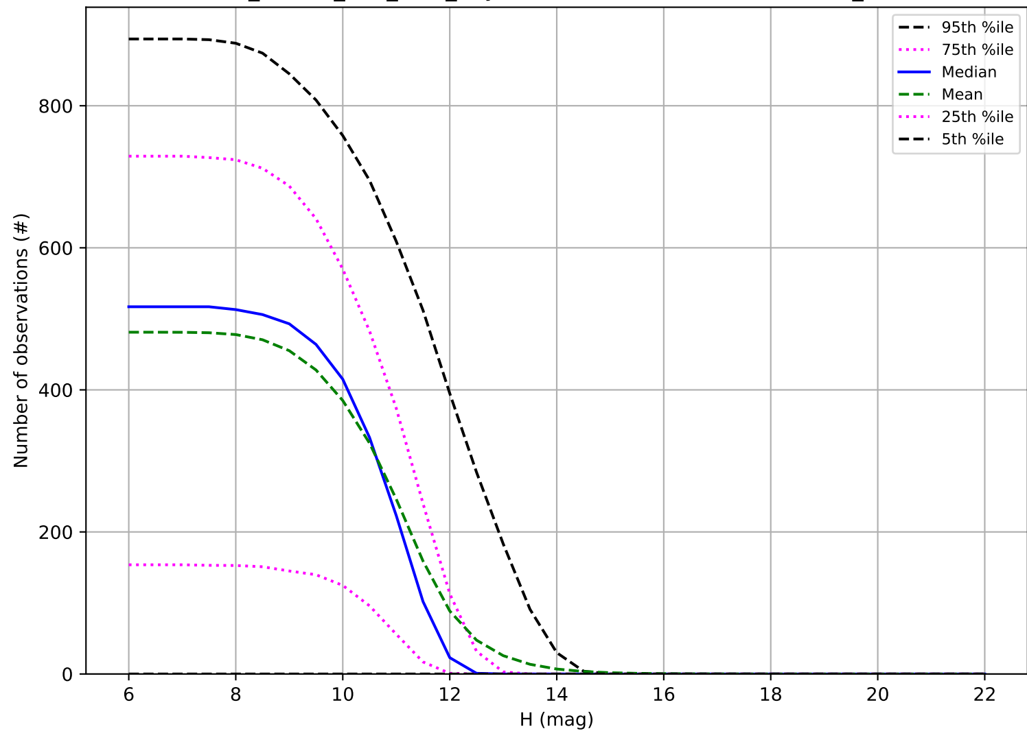
ddf_loaded_fl15_v3.4_10yrs: Number of observations OCC_r20
