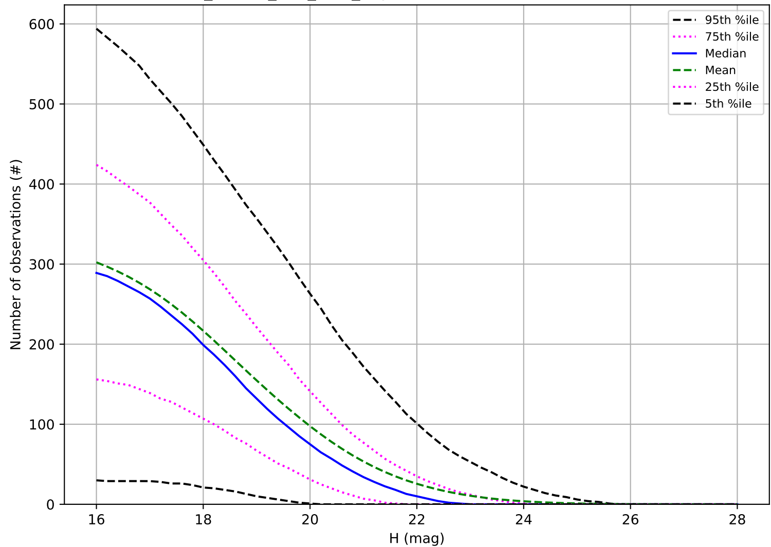
ddf_loaded_fl15_v3.4_10yrs: Number of observations NEO
