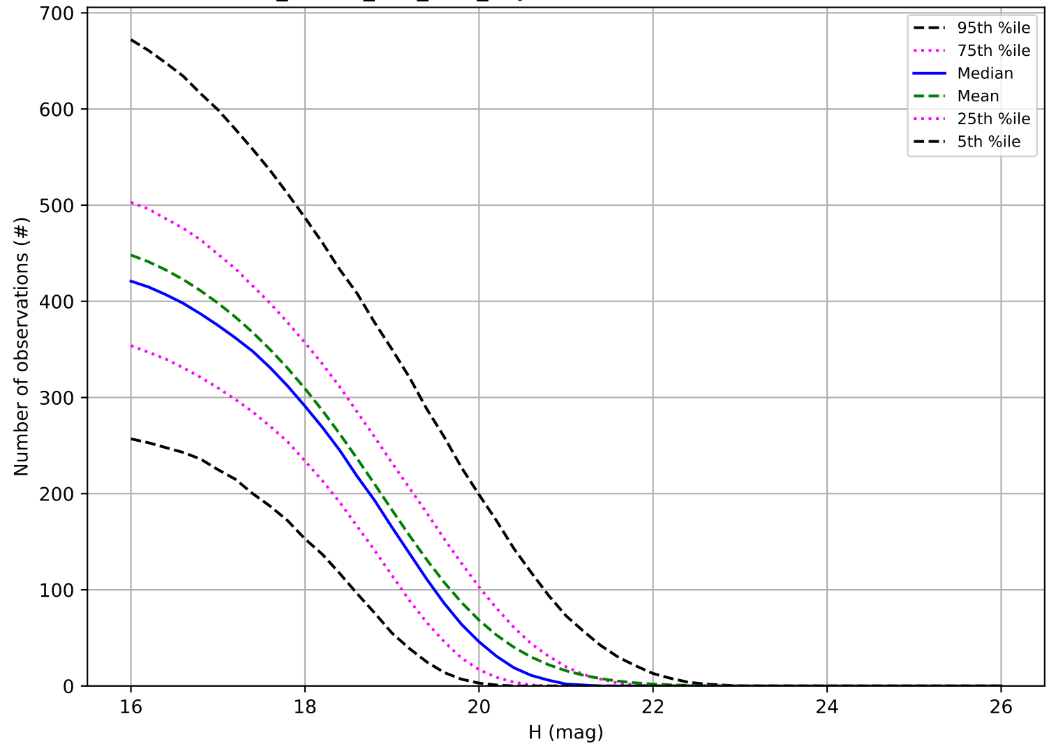
ddf_loaded_fl15_v3.4_10yrs: Number of observations MBA
