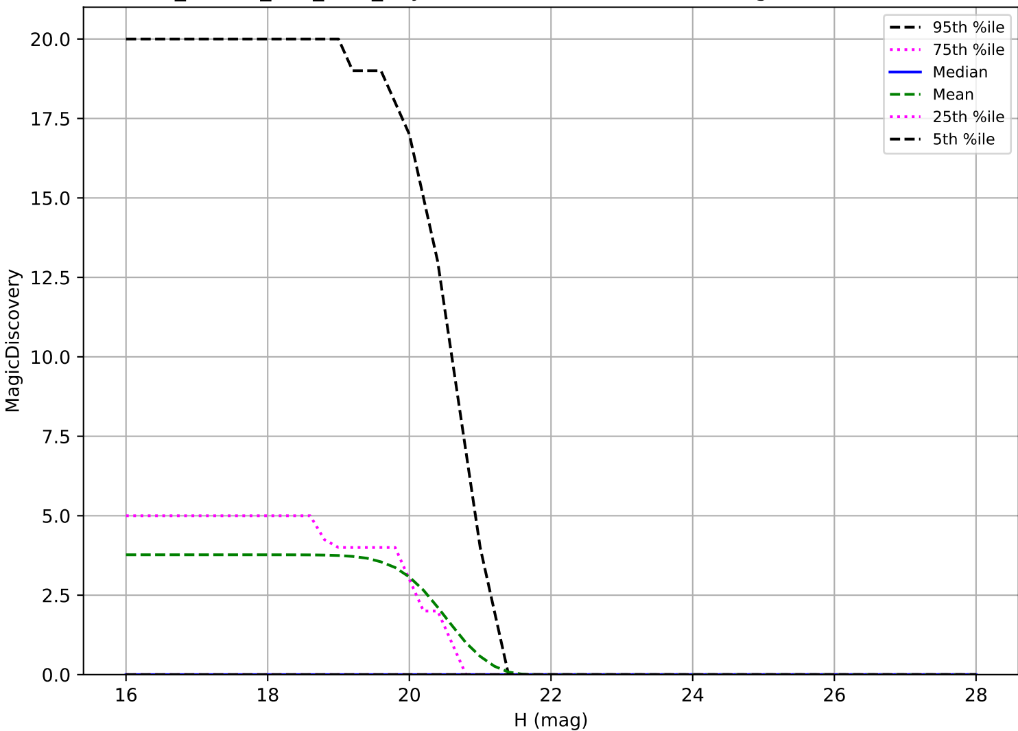
ddf_loaded_fl15_v3.4_10yrs: Vatira 6 detections in 60 nights detection loss
