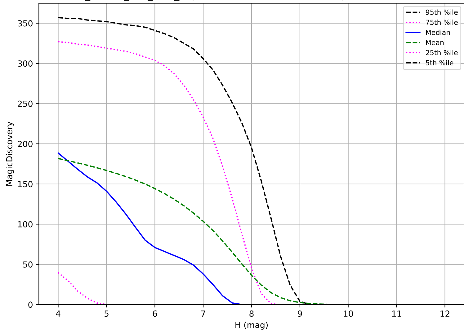
ddf_loaded_fl15_v3.4_10yrs: TNO 6 detections in 60 nights detection loss
